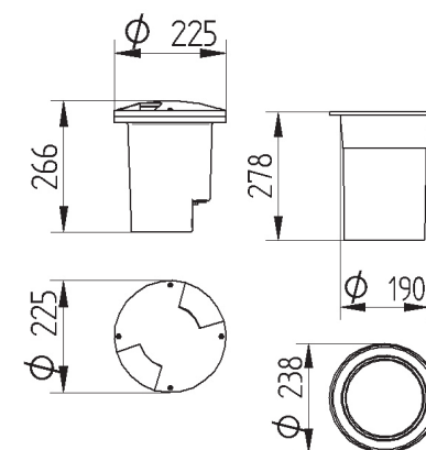
Mounting base
