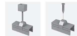
Stiff pipe with profile holder and ceiling bracket.
