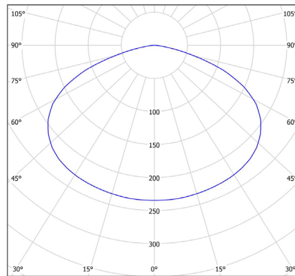
200W - 150° Optics
