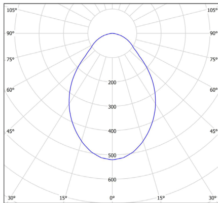
200W - 80° Optics
