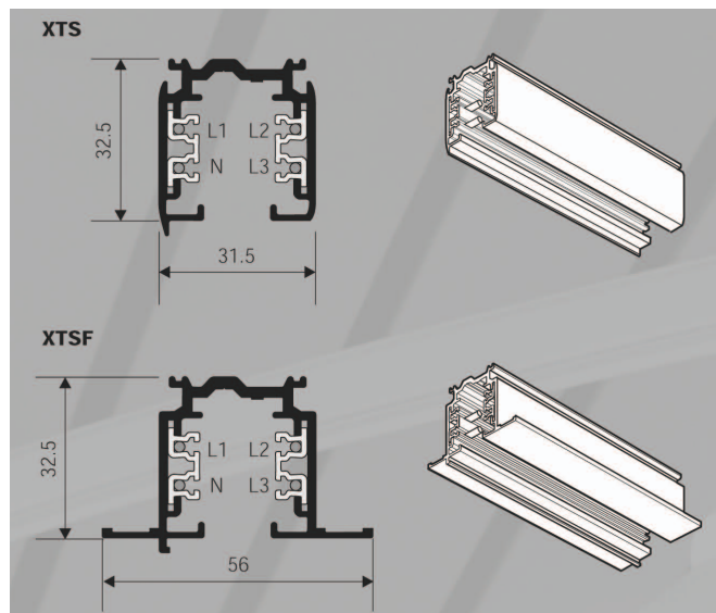
3-circuit lighting tracks (L1+L2+L3+neutral+earth) 16A/400V, Protection IP20
